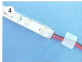
4. Put the end-cap on the end of LED strip, get the wires through the small hole.
