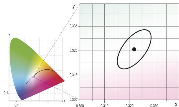
MacAdam ellipse: 3 SDCM
