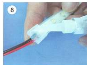
8-9. Dispense the glue on the gap between the end-cap and LED strip, and the small hole on the end-cap. Please wait for 30 minutes till the glue gets solidified.
