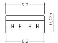
ACL plug connector PCB to PCB
