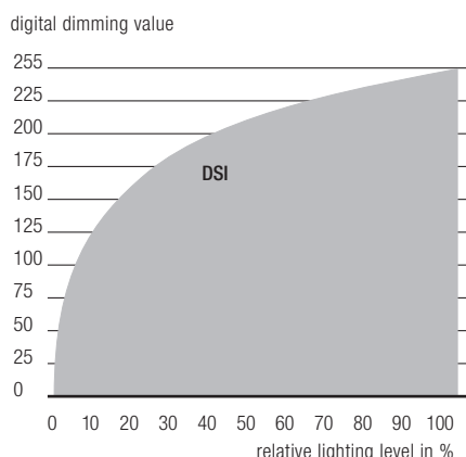
Dimming characteristics as seen by the human eye Note: The dimming level of BASIC can be different to the graphic (dimming level 10 to 100 %)
